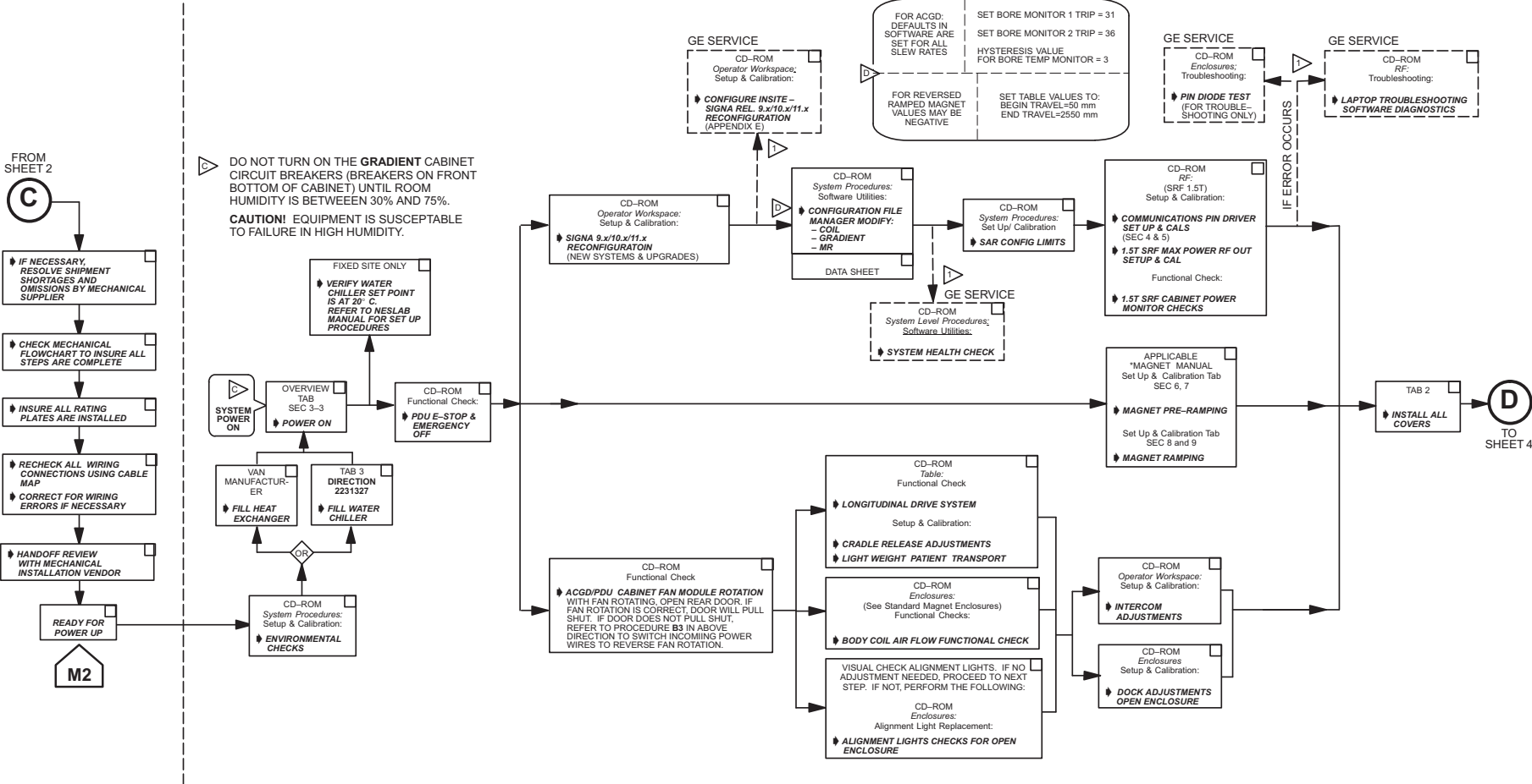
SIGNA MR/i & CV/i INSTALLATION FLOW CHART ILLUSTRATION 1-2 (SHEET 3 OF 5)
