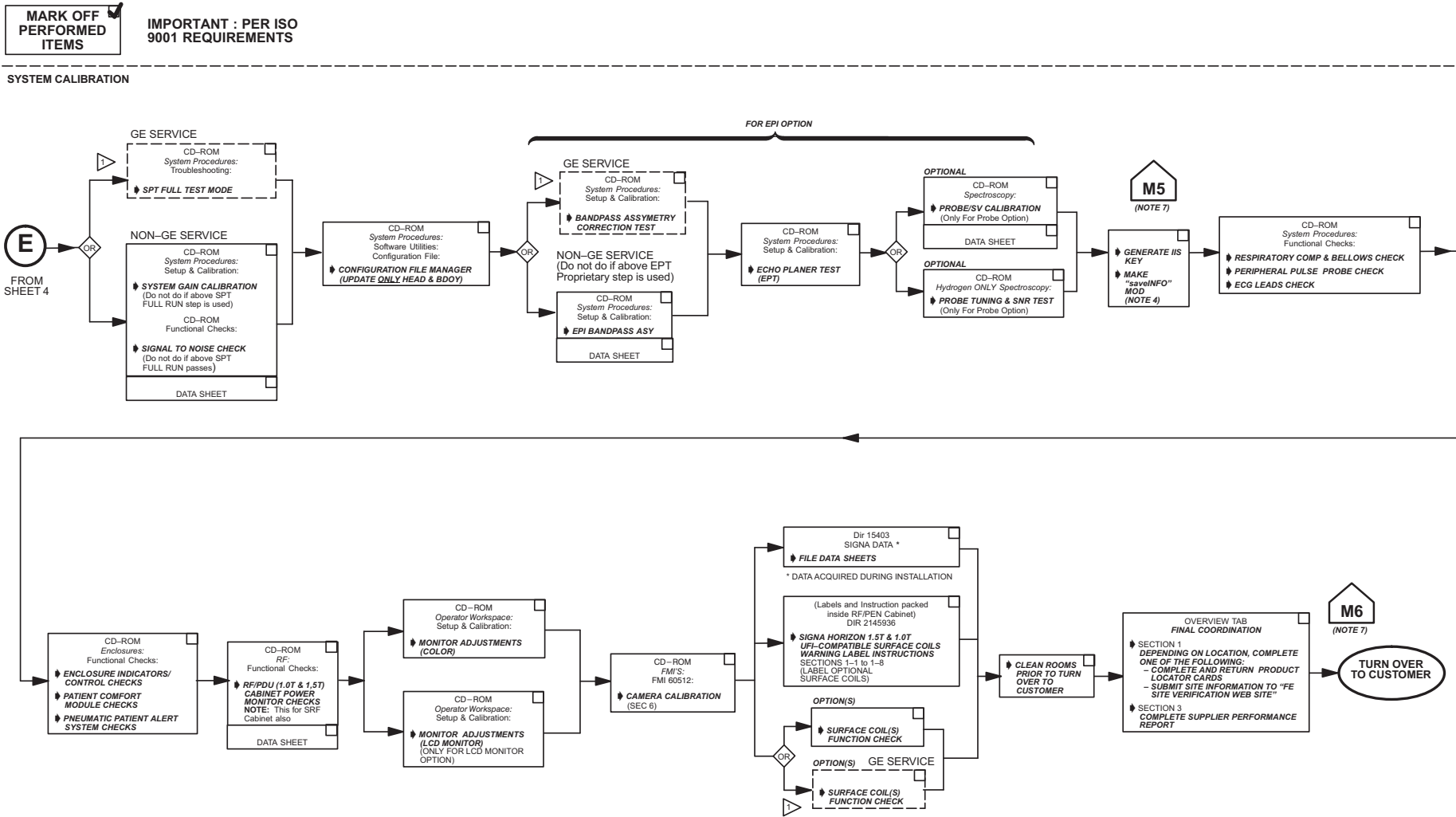
SIGNA MR/i & CV/i INSTALLATION FLOW CHART ILLUSTRATION 1-2 (SHEET 5 OF 5)
